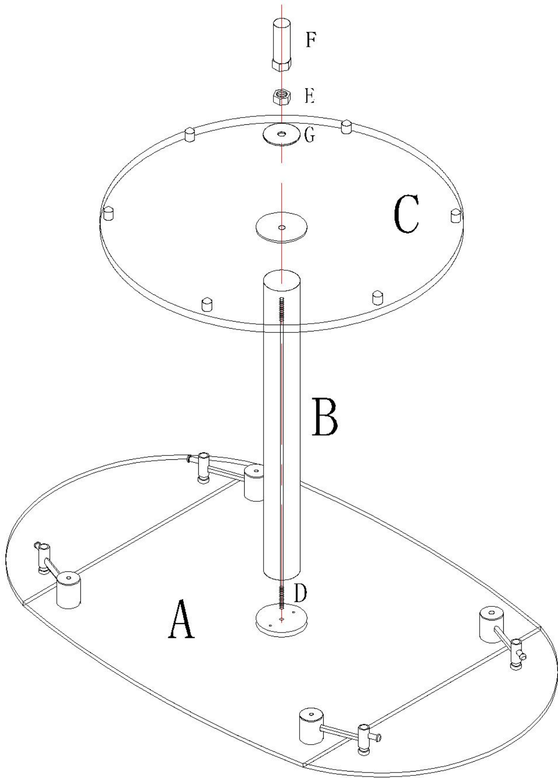
INSTALLATION DIAGRAM
